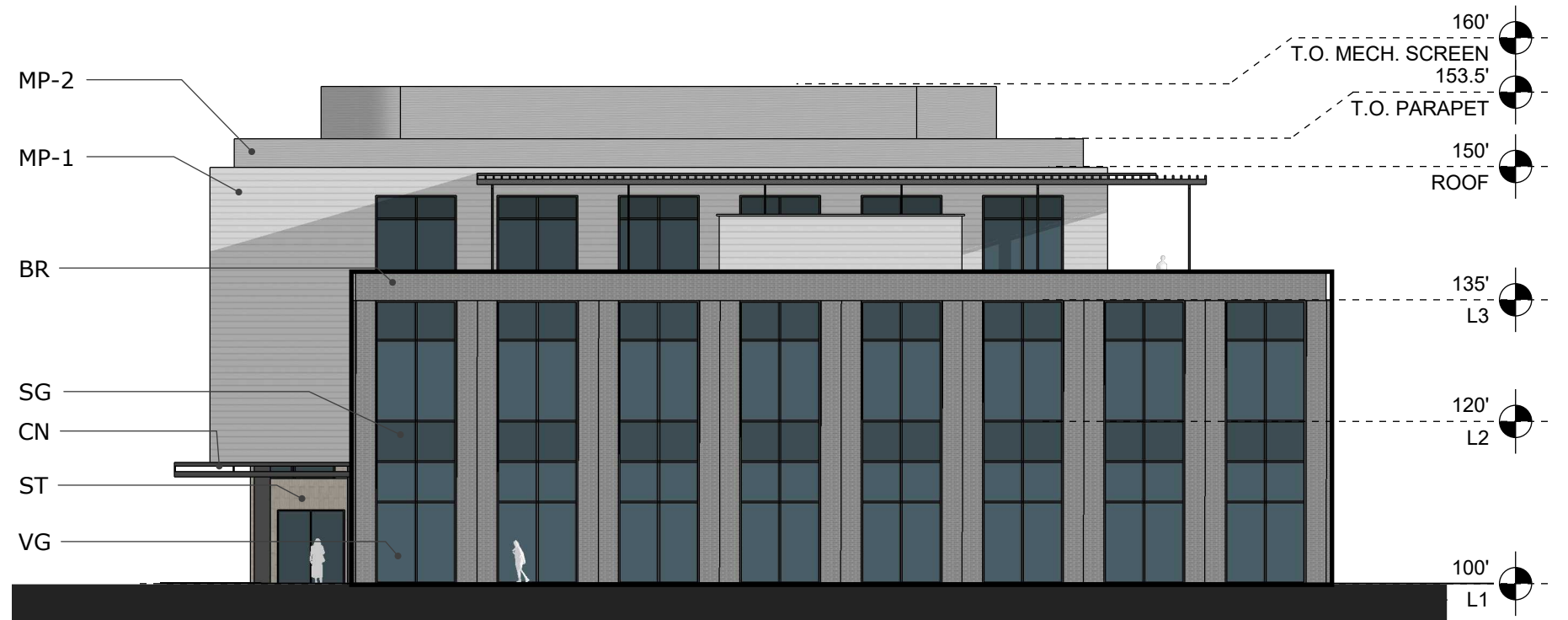
02 North Elevation Scale: 1" : 20'
